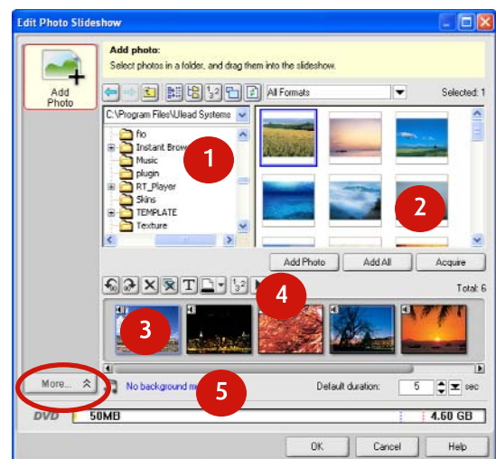
Simple Interface
