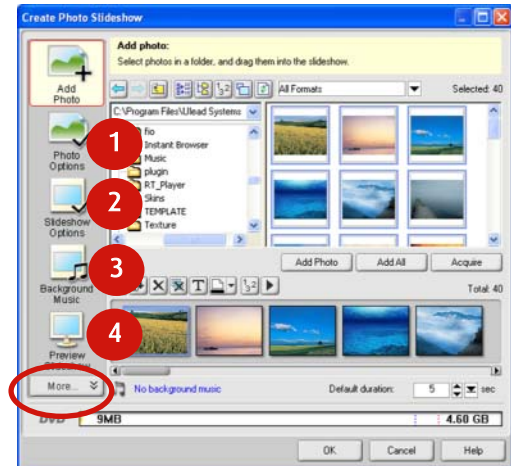
Advanced Interface
