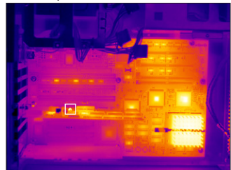
T640 - 640 x 480 pixels Max temp. 177.9°F
